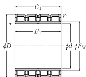
Drawings 6 to 7 2)
