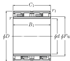
Drawings 1 to 5 2)
