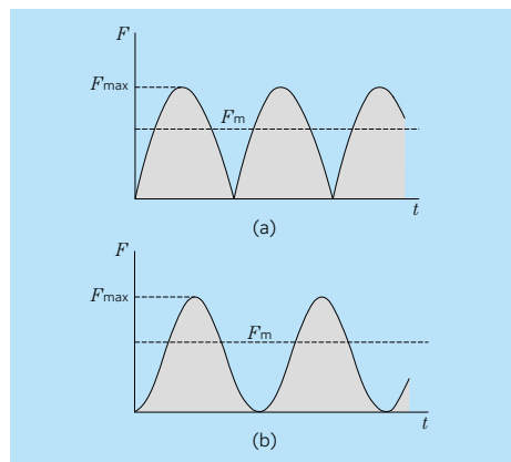
Fig. 4.14 Sinusoidal variable load
