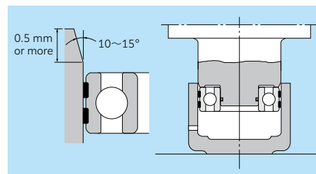
Fig. 2. Fitting method and housing inner diameter chamfer
