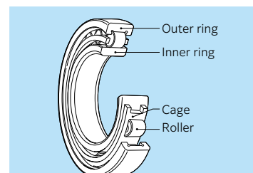
Fig. C Cylindrical roller bearing
