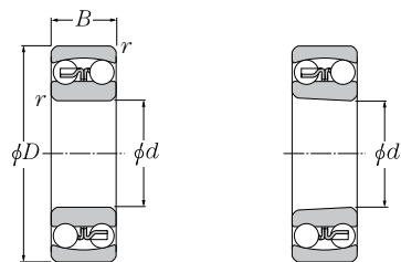
Cylindrical bore
