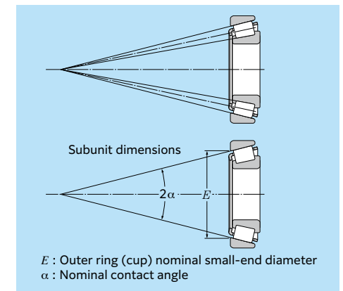
Fig. 1.5 Tapered roller bearings
