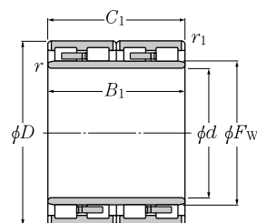
Drawings 1 to 4 2)
