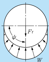
Fig. 3.10 \varepsilon = 0.5 \psi = \pm 90^\circ Radial clearance 0
