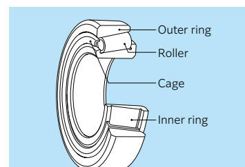
Fig. E Tapered roller bearing
